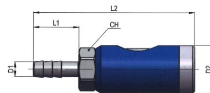
Hose stem
